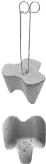
Cast concrete single spacer „THREE FEET“ with eye hook
