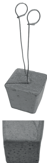
Cast concrete single spacer „SQUARE SHAPE“ with eye hook
