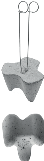
Cast concrete single spacer „THREE FEET“ with eye hook
